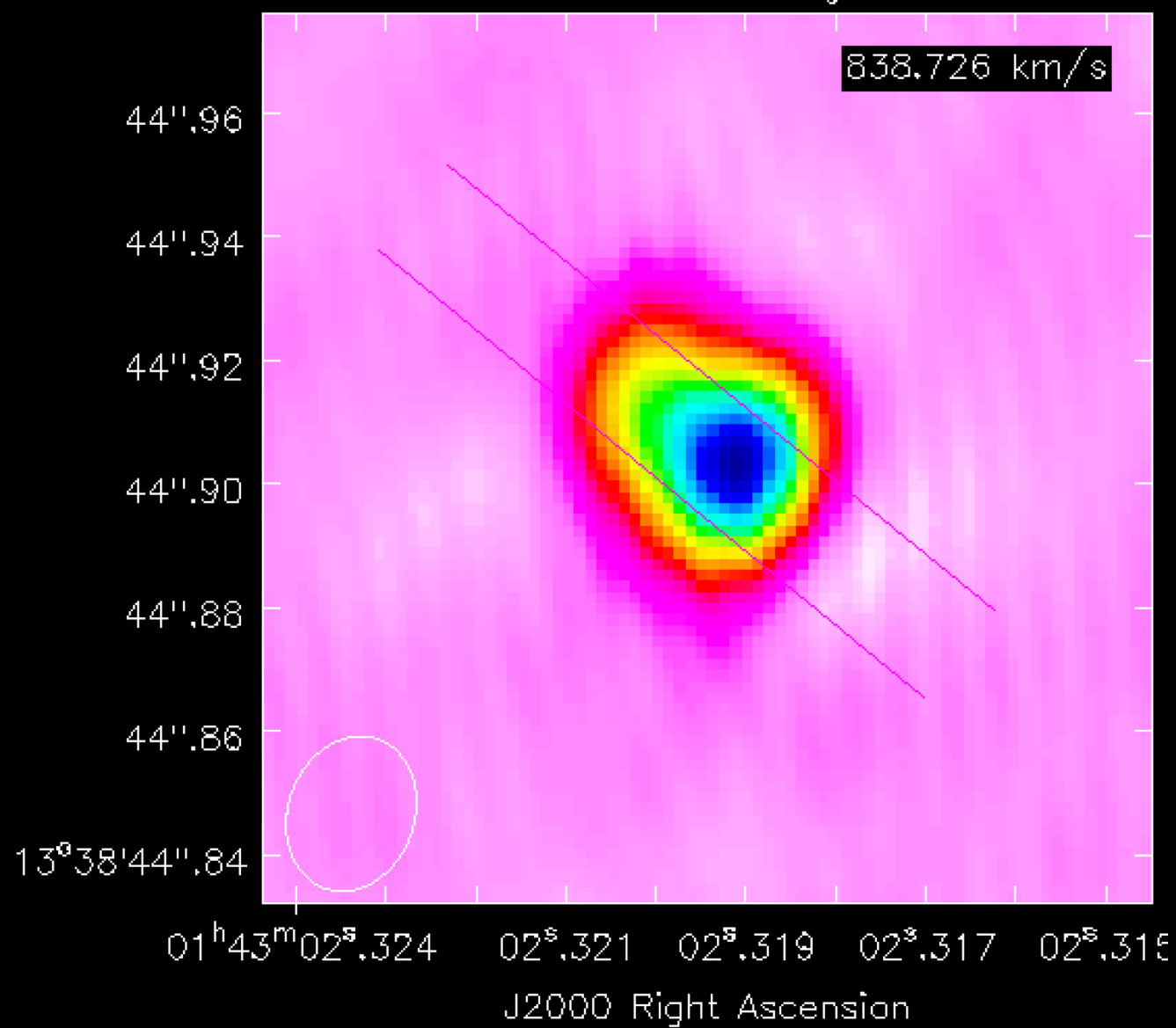
NGC660_line.clean.image-raster
