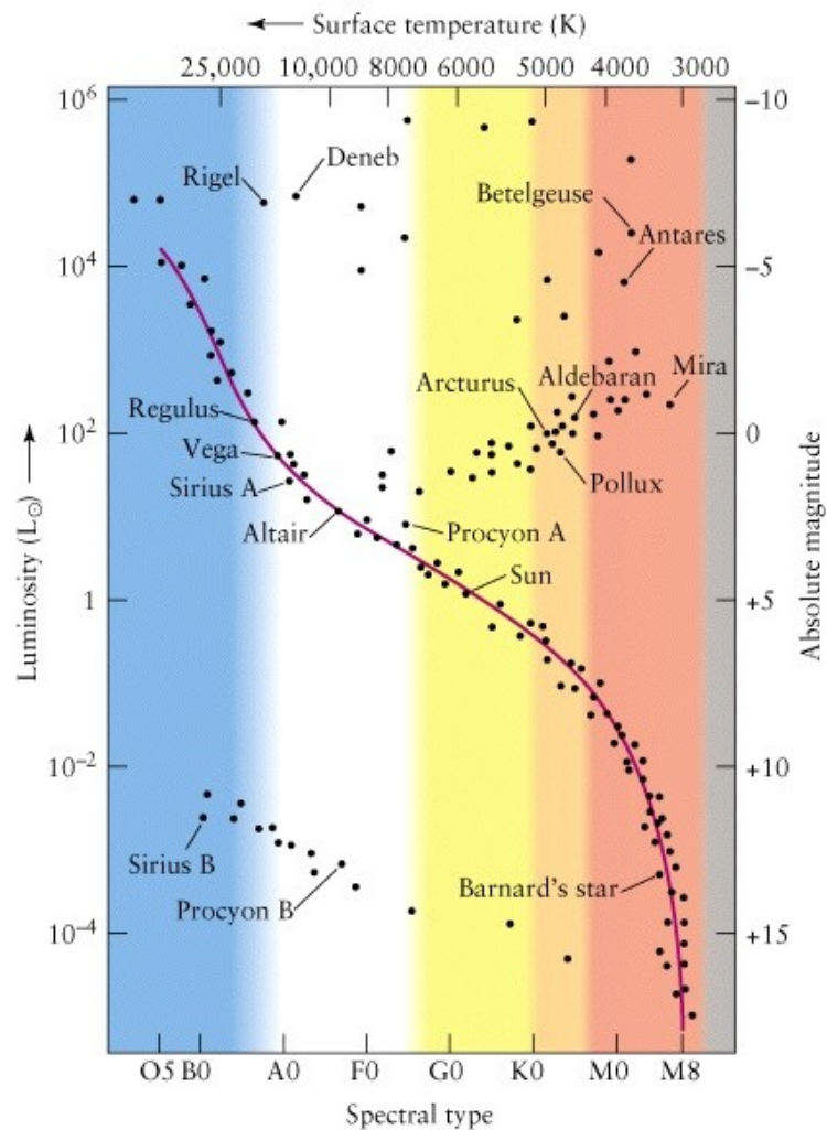
H-R diagram for some bright stars
