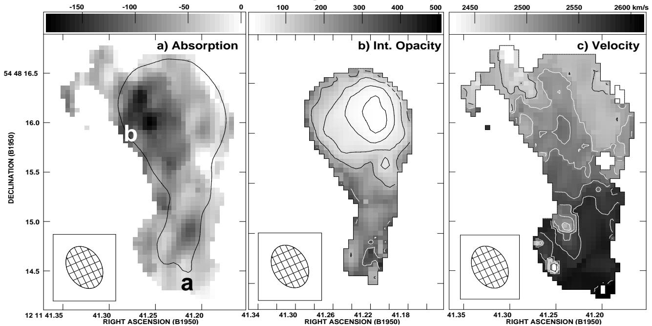
Fig. 4. a) The (leftmost) image shows the integrated H \alpha absorption signal across the centre of the Medusa merger. This has been derived from the continuum subtracted spectral line cube. The grey-scale flux density range is 0 \rightarrow -185 \text{ mJy km}^{-1} . Note the absorption shown is dependent on the strength of the continuum emission. The two symbols (a and b) shown on the left-most image represent two of the CO emission peaks from AH00. A single contour 1 \text{ mJy beam}^{-1} radio continuum contour is overlaid. Areas external to this contour have the lowest levels of radio continuum and have been excluded in the derivation of Fig 4b. b) The (central) image shows the integrated optical depth ( \int \tau dV ) across the same region as a . The grey-scale range shown is 15 \rightarrow 500 and the contour levels are 10, 20, 40, 80, 160, 320 and 640 times 100. It should be noted that errors in this image increase in areas where the radio continuum flux density is at a minimum. This effect results in some erroneous values toward the edges of the image, in order to remove the most severe of these effects this image has been blanked in areas where the radio continuum is less than 1 \text{ mJy beam}^{-1} . c) The (right-hand) map represents the H \alpha absorption velocity field over areas where significant radio continuum and absorption line signal were detected. The grey scale range of the image is 2430 \rightarrow 2610 \text{ km s}^{-1} , the overlaid contours have increments of 25 \text{ km s}^{-1} between 2475 \rightarrow 2650 \text{ km s}^{-1} .
