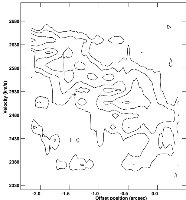
Fig. 5. A position velocity diagram of H \alpha absorption in the central region of the Medusa merger. The absorption has been averaged over the entire R.A. range of the radio source, where the radio continuum is in excess of 0.6 \text{ mJy beam}^{-1} . The contour levels are set at -8 , -5.657 , -4 , -2.282 , -2 , -1.414 , -1 and 1 times 0.36 \text{ mJy beam}^{-1} . The position axis is declination relative to 54^\circ 48' 16''.4 .
