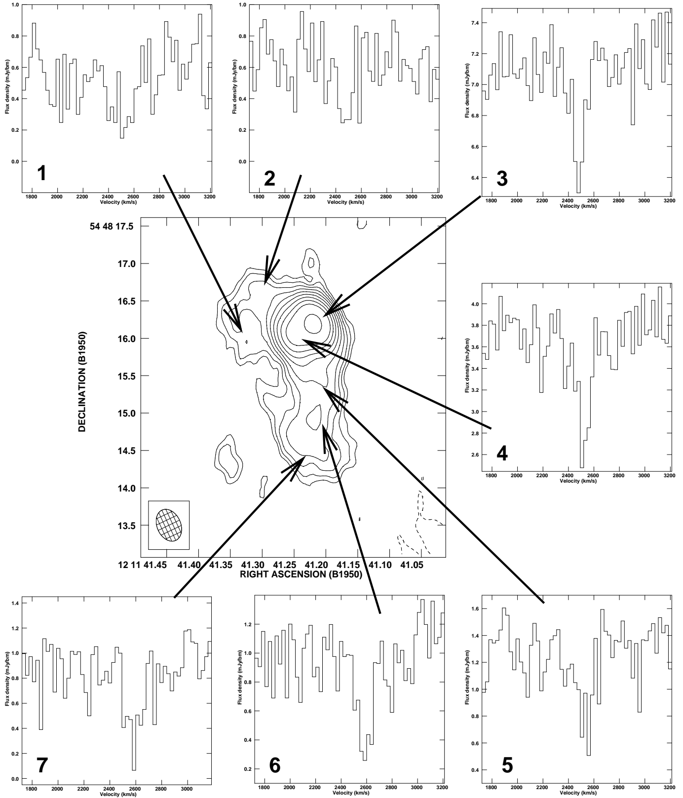
Fig. 3. Montage of 800-k \lambda uv -tapered radio continuum structure and H I absorption spectra. Contour levels of the central image start at 0.3 mJy \text{bm}^{-1} and increase by factors of \sqrt{2} with an angular resolution of 0''.45 \times 0''.32 .
