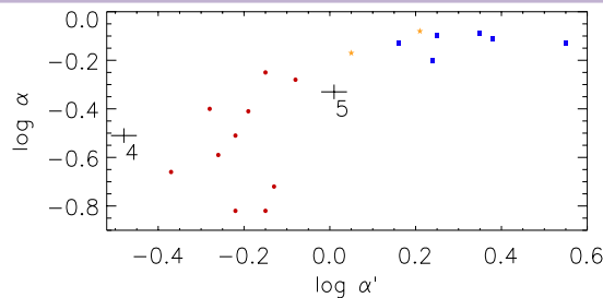
Figure 2. The spectroscopic criteria, \alpha and \alpha' , are plotted with errors (black crosses) for the target stars for which we currently have spectra. They are labelled numerically as in Fig. 1 and plotted alongside a sample of stars presented in Smith (1970). In this reproduction, the Am stars are red circles, the normal stars are blue squares, and the objects represented by orange star-shaped symbols have been classified as Am and normal in two separate studies.
