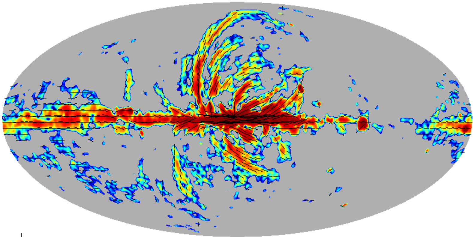
WMAP-K Pol. Amp + B-field vectors
