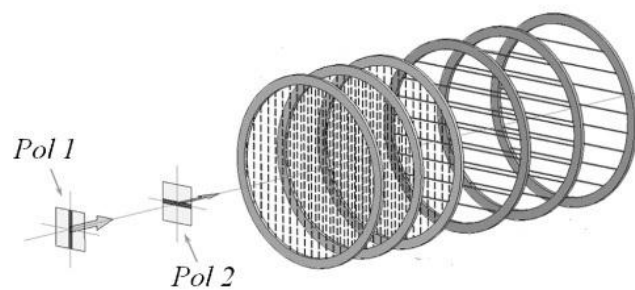
Half-wave plate
